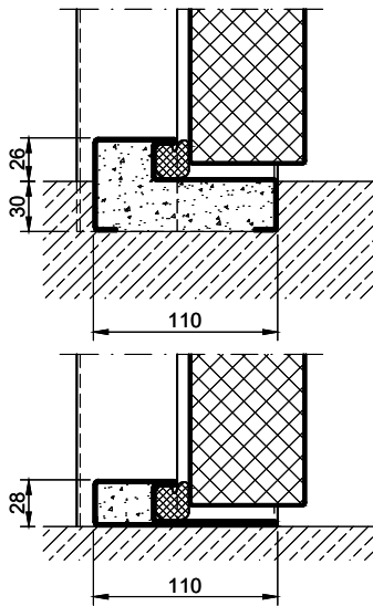
separation sill with half sill
