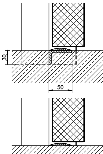
separation sill with half sill
